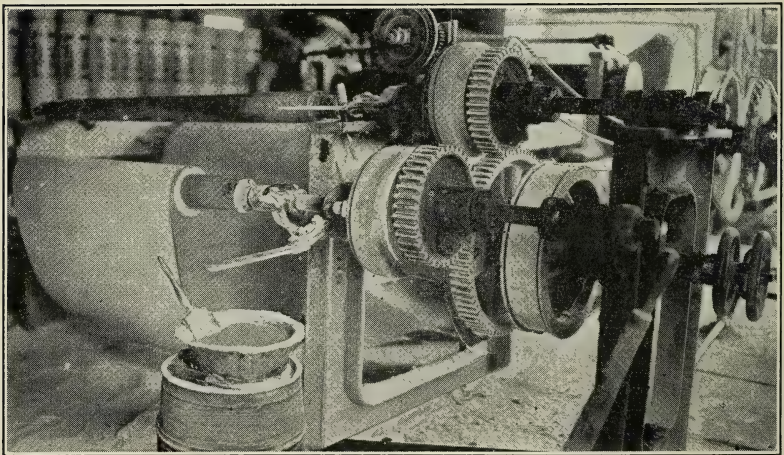
FIG. 131.—Winding Mechanism.
